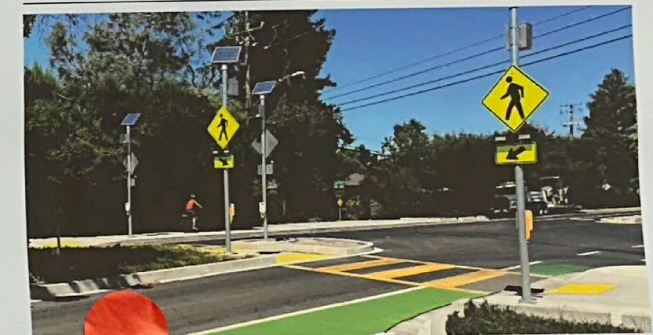
Rectangular Rapid Flashing Beacon
