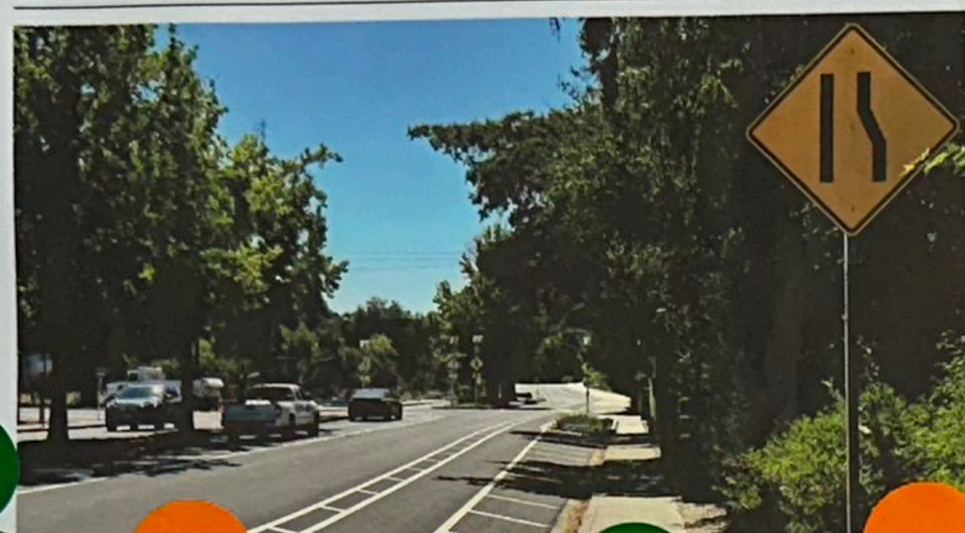
Buffered Bike Lane
